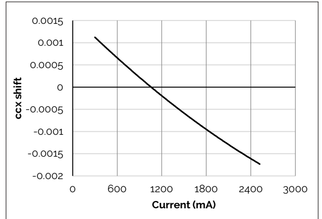
Figure 14: V22D Drive Current vs. ccx Shift
