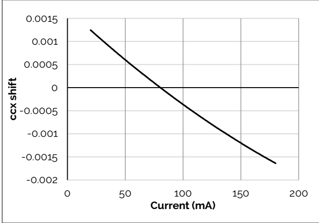
Figure 14: V6C Drive Current vs. ccx Shift
