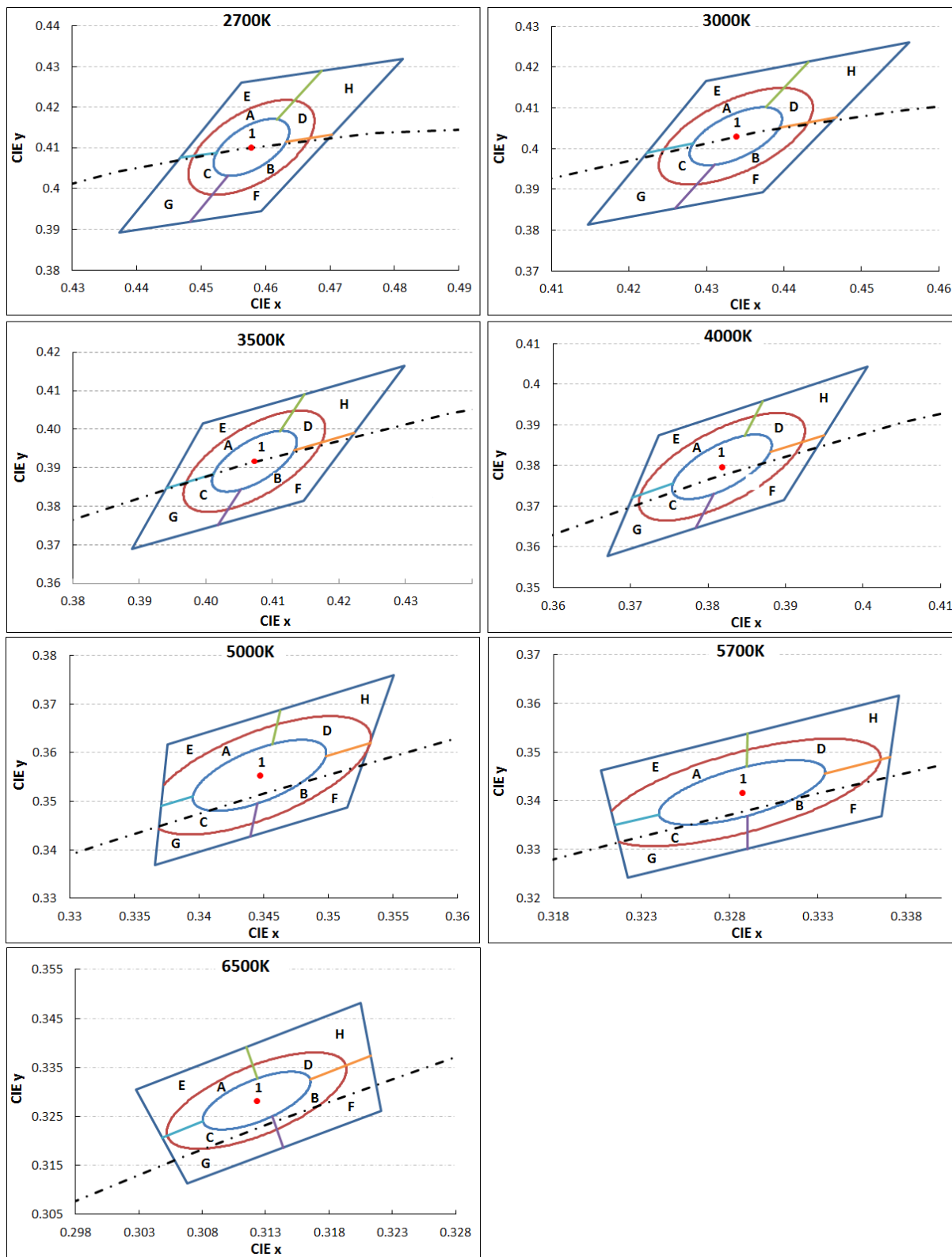
Figure 1: C.I.E. 1931 Chromaticity Diagram (g Color Bin Structure, hot-color targeted at T_{sp} = 85^{\circ}\text{C} )
