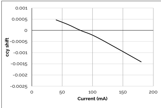
Figure 7: V6C Drive Current vs. ccy Shift
