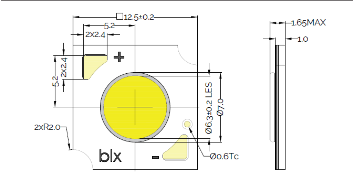
Figure 12: Drawing for V6 LED Array
