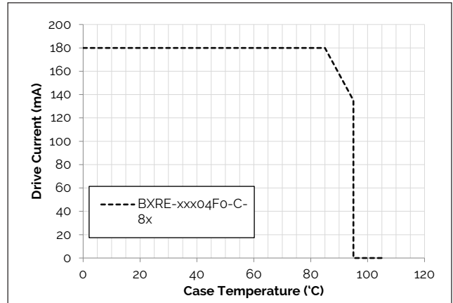
Figure 8: Derating Curve
