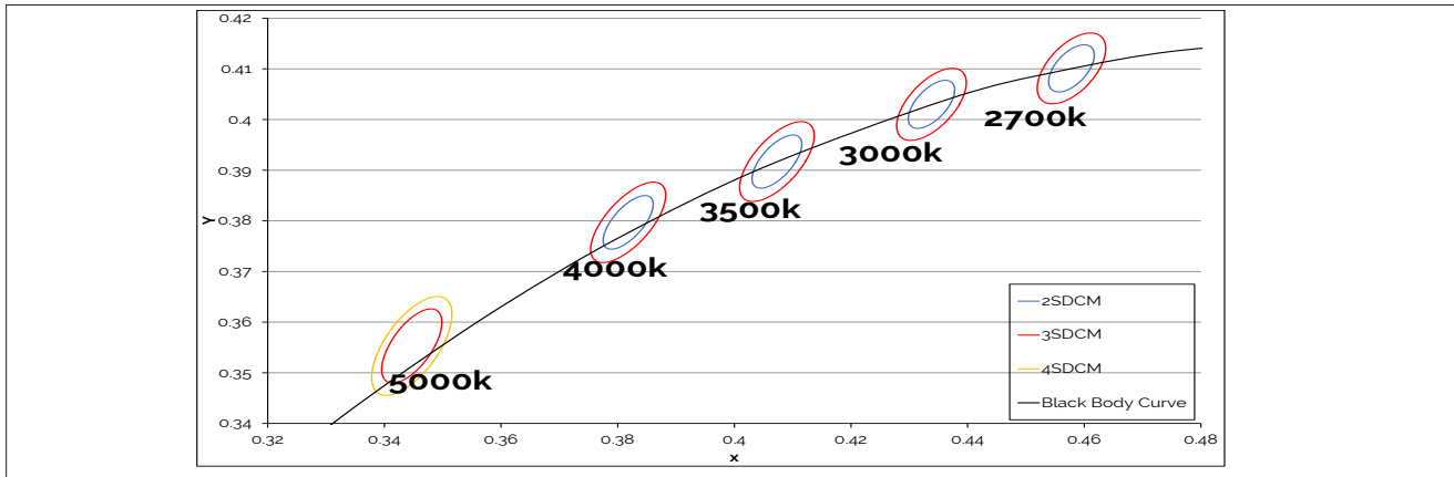
Figure 13: Warm, Neutral and Cool White Test Bins in xy Color Space
