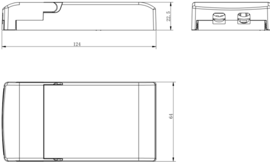
Figure 5: Mechanical Drawing
