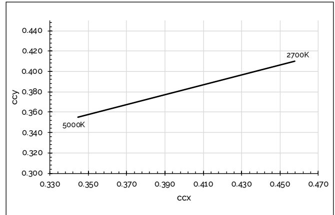
Figure 12: CCT Tuning Range, Tc=85°C
