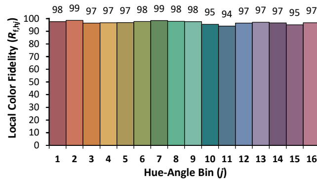
Figure 3: 6500K Thrive TM-30 Graphs
