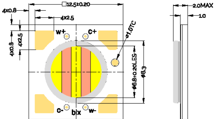
Figure 18: Mechanical Drawing Specifications BXRV-TR-27XXX-06A0-B-2X
