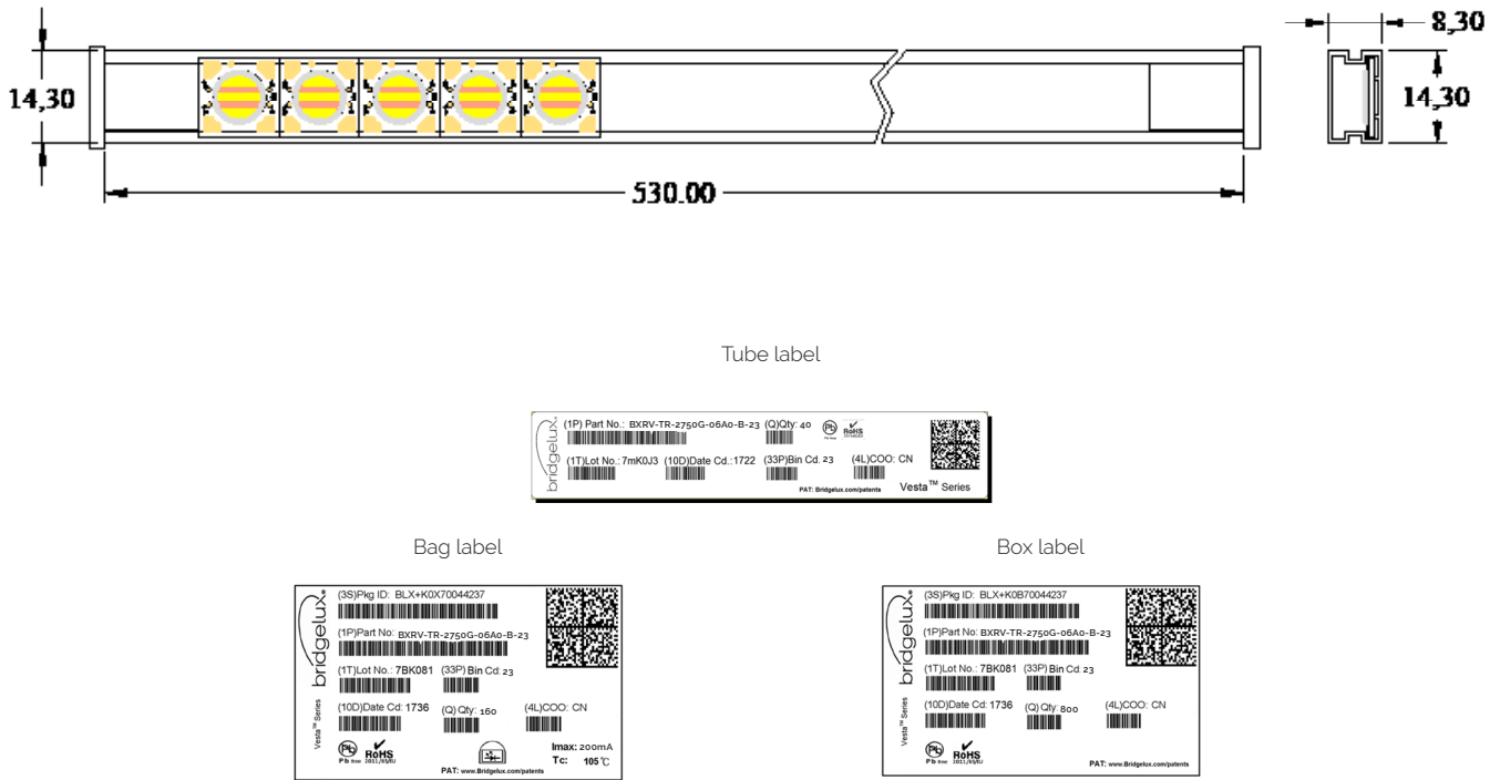
Figure 21: Vesta Series Tunable White 6mm Packaging and Labeling
