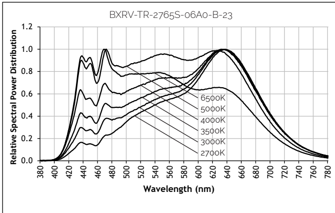
Figure 17: 2700K - 6500K with Thrive
