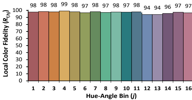
Figure 2: 5000K Thrive TM-30 Graphs
