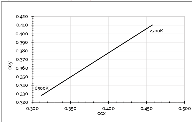
Figure 13: CCT Tuning Range, Tc=85°C
