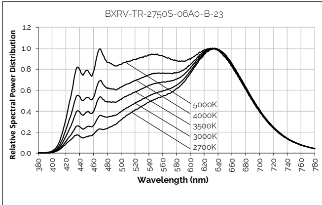
Figure 16: 2700K - 5000K with Thrive
