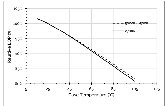
Figure 8: Relative Light Output vs. Case Temperature
