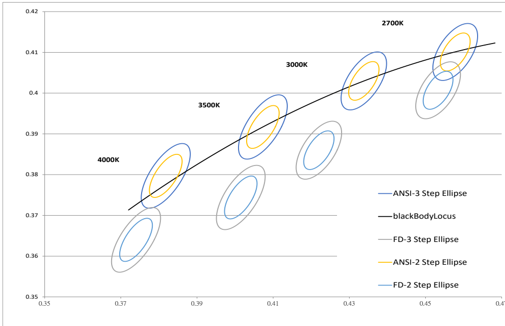
Figure 11: Warm and Neutral White Test Bins in xy Color Space
