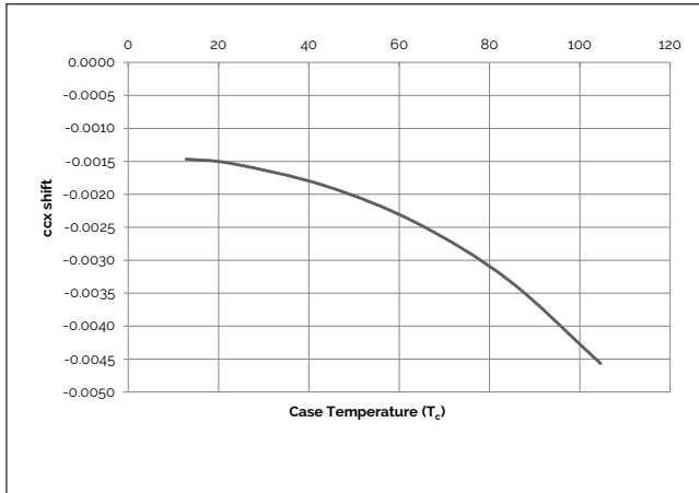
Figure 6: Typical DC ccx Shift vs. Case Temperature 4
