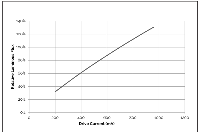
Figure 4: Typical Relative Flux vs. Current V6G HD 1,2
