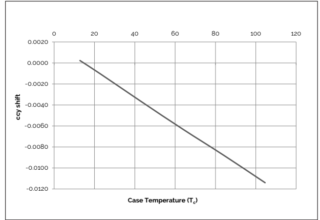
Figure 7: Typical DC ccy Shift vs. Case Temperature 4
