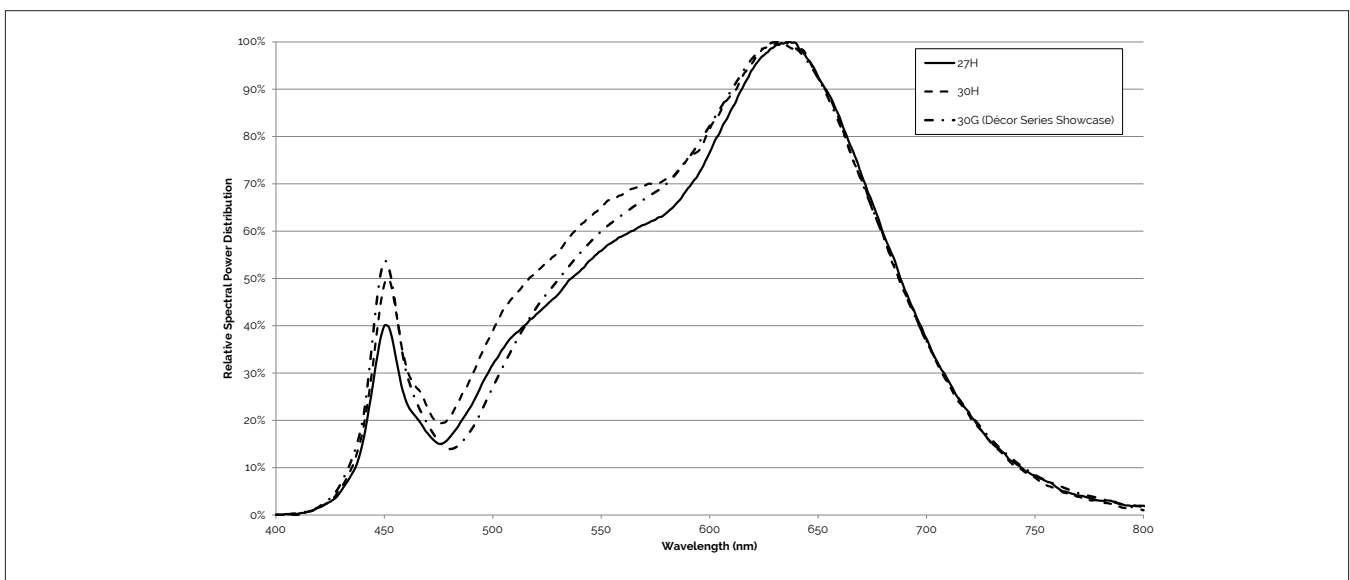
Figure 15: Typical Color Spectrum for Décor Series
