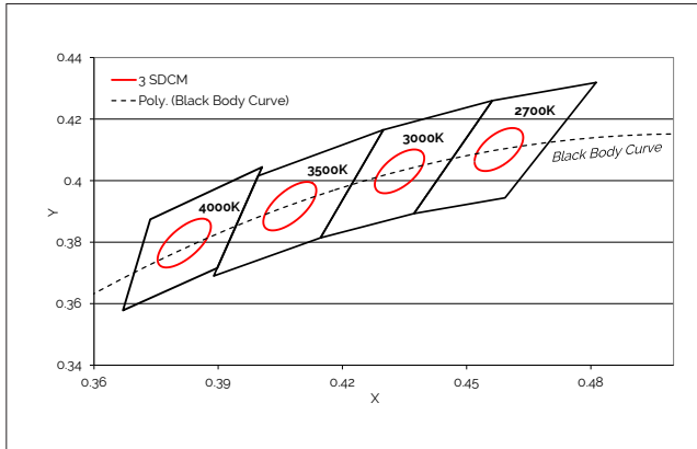
Figure 17: Warm and Neutral White Test Bins in xy Color Space
