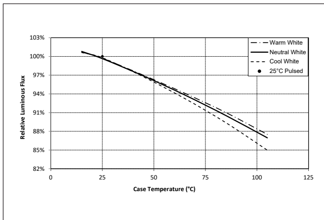
Figure 5: Typical DC Flux vs. Case Temperature 3
