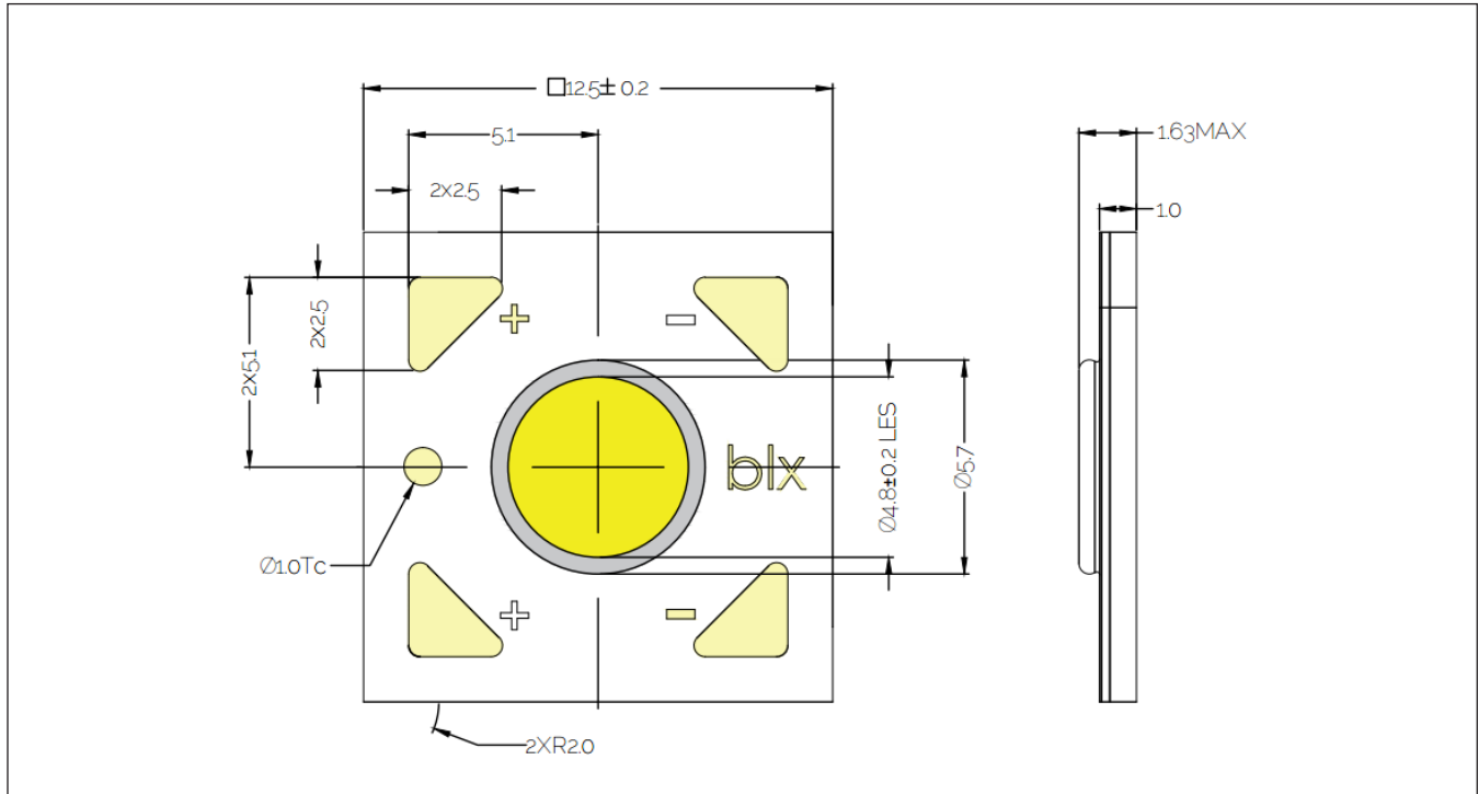
Figure 14: Drawing for V4 HD LED Array
