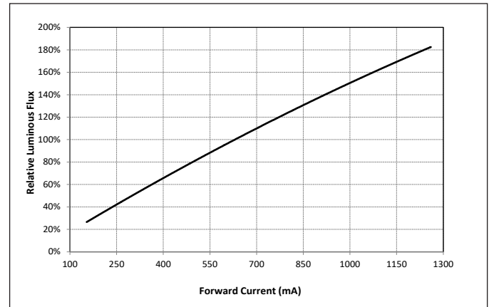
Figure 12: Vero SE 13C Typical Relative Flux vs. Current ( T_c=25^\circ\text{C} )
