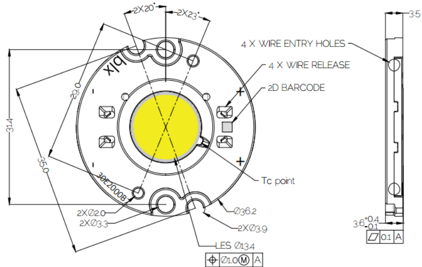
Figure 18: Drawing for Vero SE 13 LED Array
