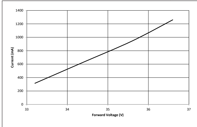
Figure 11: Vero SE 13C Drive Current vs. Voltage ( T_c=25^\circ\text{C} )
