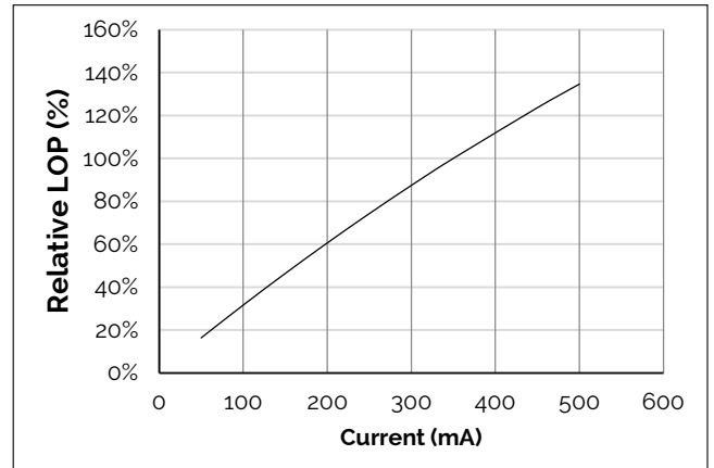
Figure 2: V6C HD Typical Relative Flux vs. Drive Current ( T_j = T_c = 25^\circ\text{C} ) 1
