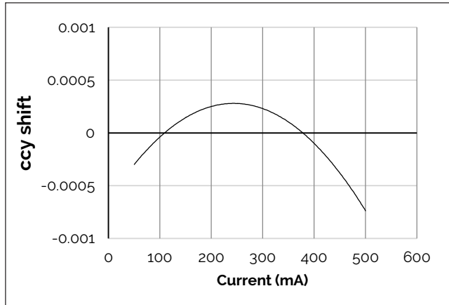
Figure 7: V6C HD Drive Current vs. ccy Shift
