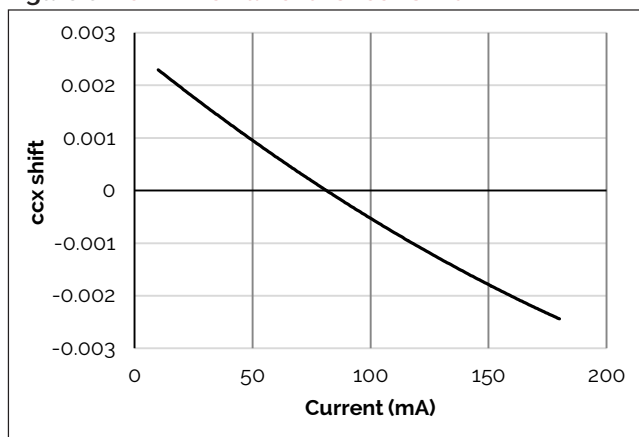
Figure 6: V6C Drive Current vs. ccx Shift
