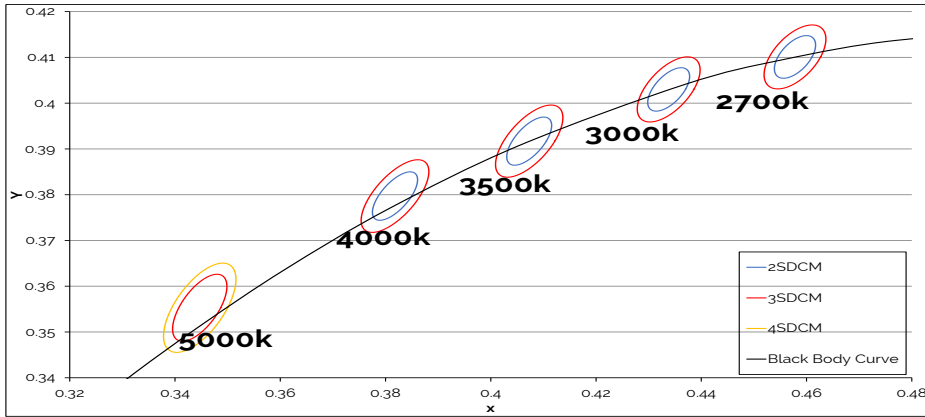
Figure 11: Warm, Neutral and Cool White Test Bins in xy Color Space
