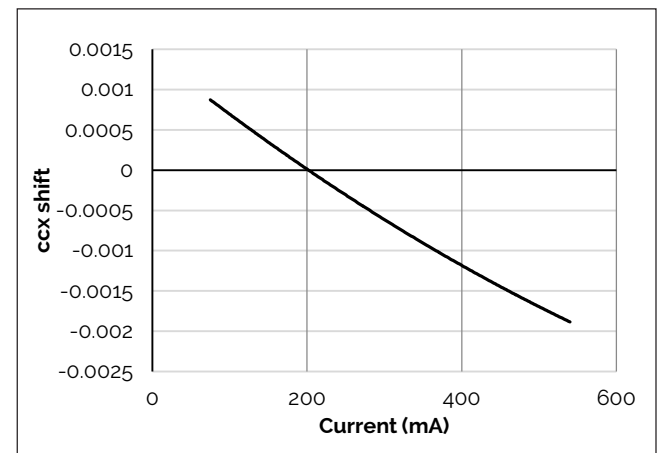
Figure 6: Vero10B Drive Current vs. ccx Shift
