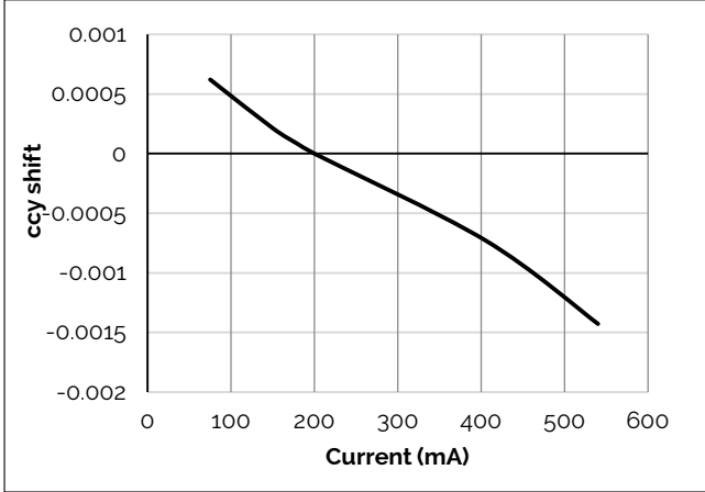
Figure 7: Vero10B Drive Current vs. ccy Shift
