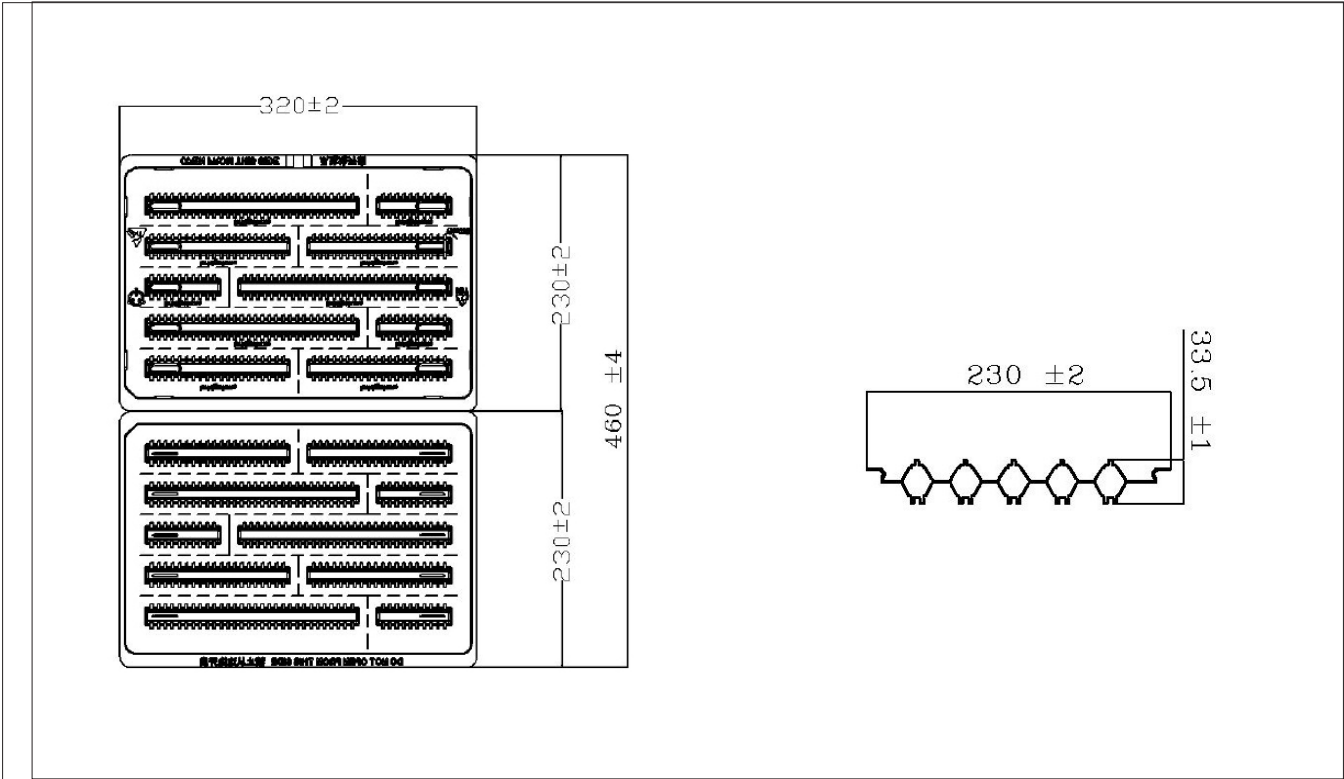
Figure 13: Drawing for Vero 10 Packaging Tray
