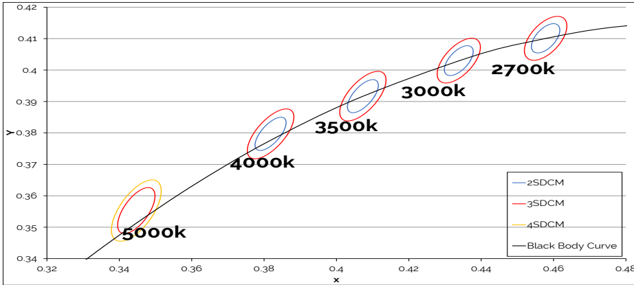
Figure 12: Warm, Neutral and Cool White Test Bins in xy Color Space
